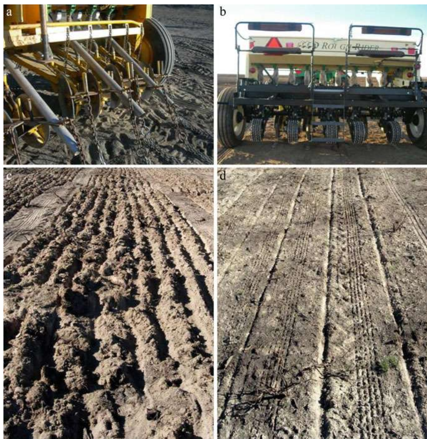
Fig. 5.5 Rangeland drills are designed to seed multiple species at different depths of soil. Traditional rangeland drill (a) that places seeds in furrows (c). In contrast, minimum-till rangeland drill (b) leaves the soil flat (d) after placing seeds. Photo credits. a, b, c and d. Location likely Mountain Home, Idaho in 2006. Photo by US Forest Service. Image currently on Great Basin Fire Science Exchange, Revegetation Equipment Catalog, but originally in Joint Fire Science Final Report, Project #07-1-3-12 by Dr. Nancy Shaw, USFS, https://www.fs.usda.gov/rm/pubs_other/rmrs_2011_shaw_n003.pdf . Photo now found on https://revegetation.greatbasinfirescience.org/wp-content/uploads/2021/01/LRangelandDrillRightMinTillDrill_SoilDisturbance_USFS-294x300.jpg
